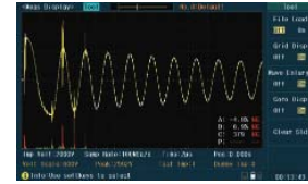
Corona display in magnified waveform display
