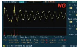
Corona display in normal waveform display
