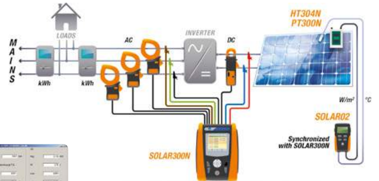
Connection diagram (three-phase system)
